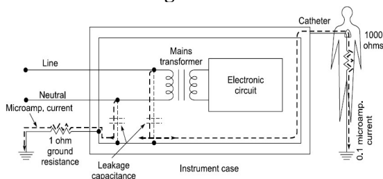
Path of leakage current in a normal case of discontinuous ground
