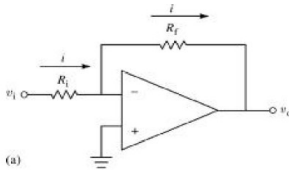
Inverting Amplifier
