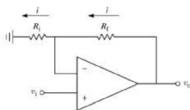
Non-Inverting Amplifiers
