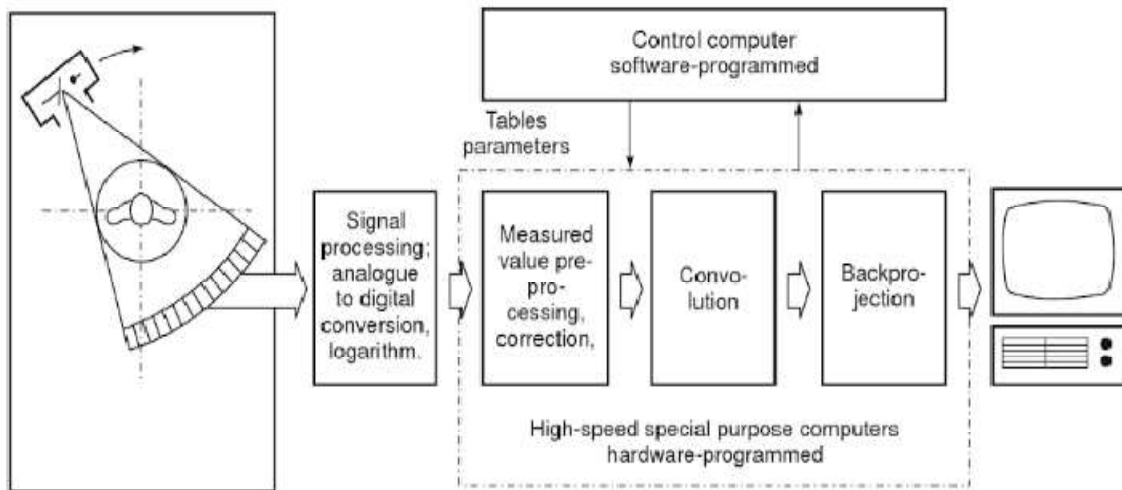
► Fig. 20.13 Block diagram of the image computer. The synchronous reconstruction of the image permits the representation of the tomogram on the video monitor immediately upon completion of the scan (Courtesy: Siemens, Germany)
