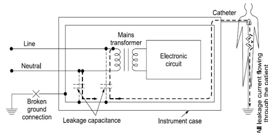
Path of leakage current in case of broken ground connection
